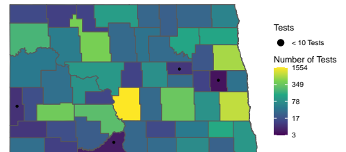
Figure 9: Smoothed number of Radon tests by county.
